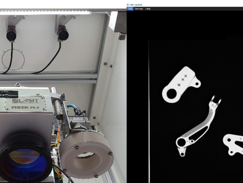
Fig. 2: Array of cameras installed inside the LASIT marking machine, GUI of the MUSP Software for machine control and piece recognition
