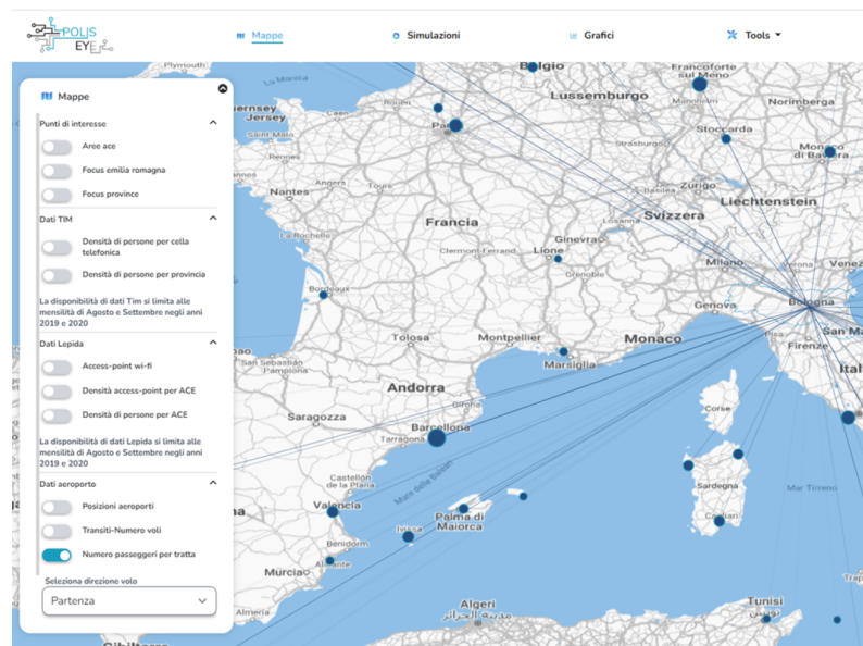
Fig. 1: Dashboard
