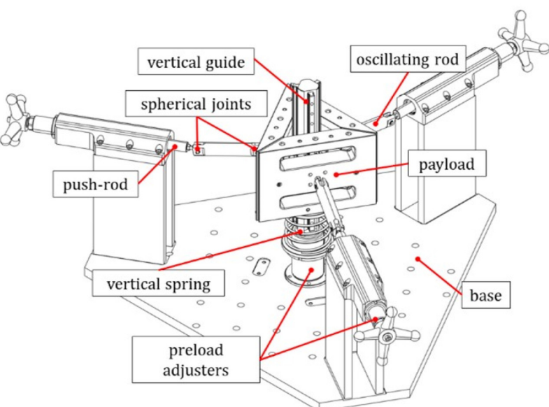
Fig. 2: Tripod isolator with HSLDS characteristics
