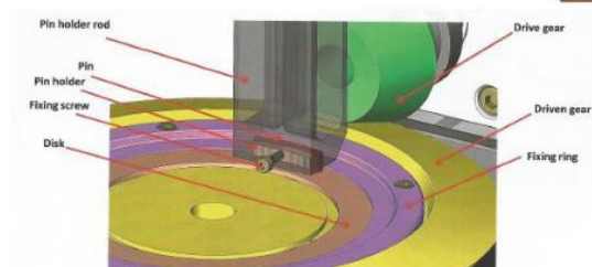
Fig. 1: Macchina test pin on disk FM Lab.
