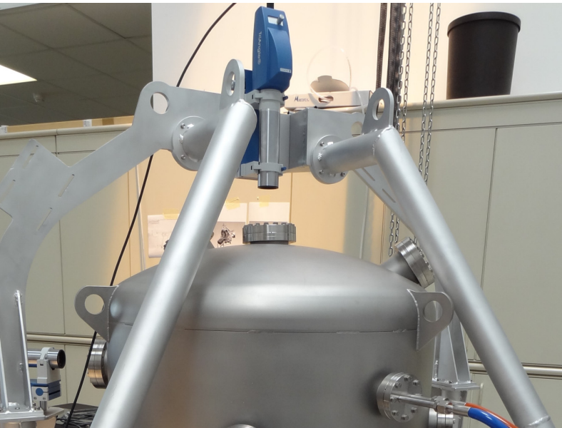
Fig. 3: Optical measurements with autocollimators mounted on GSE windows
