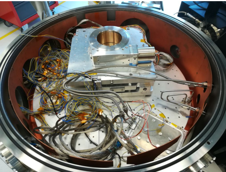
Fig. 2: GSE inside view with cold plates and 3-axes micro positioning system
